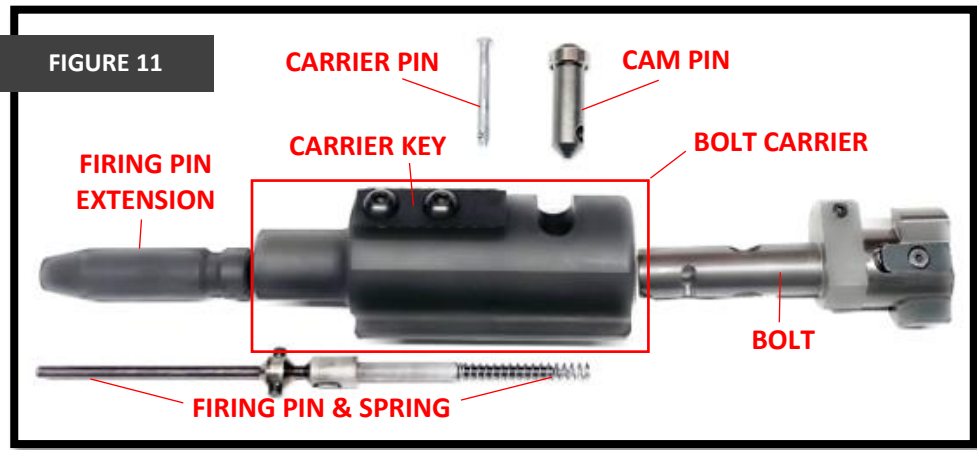
Figure 11: Disassembled Bolt Carrier. Shown above are the disassembled components of the Bolt Carrier Group.
